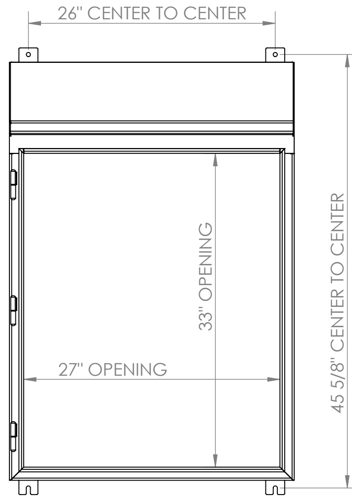
DOOR HIDDEN TO SHOW PANEL OPENING
